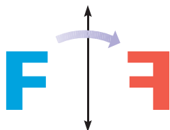
Reflection in a line
