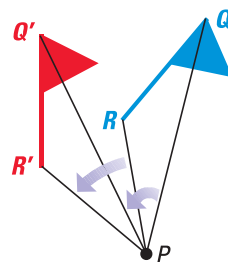
Counterclockwise rotation of 40^\circ
